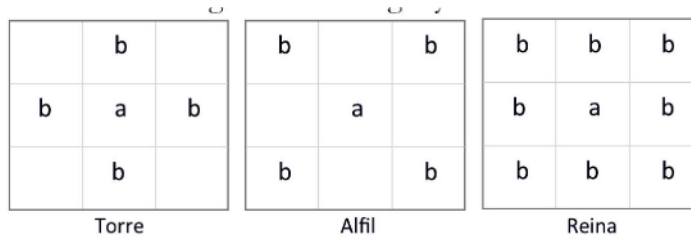
Fig. 2. Contiguity matrix
